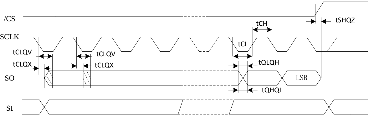
Figure 38. Output Timing
