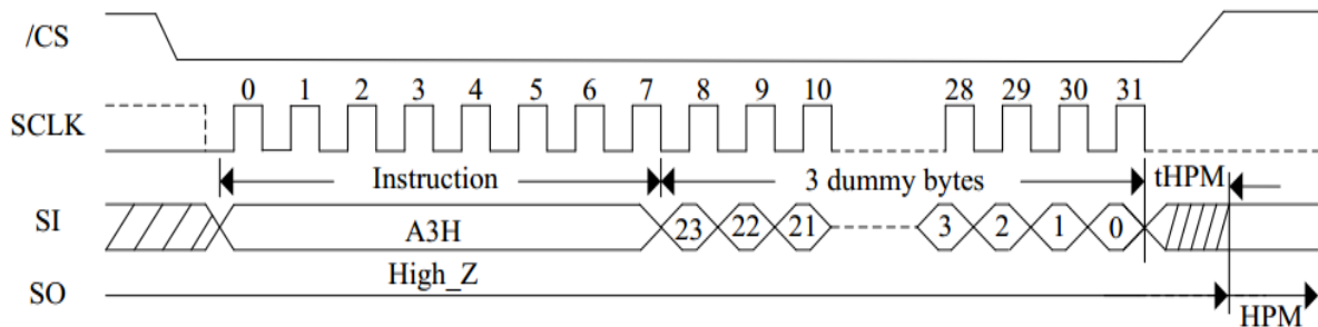
Figure 43. High Performance Mode Sequence Diagram
