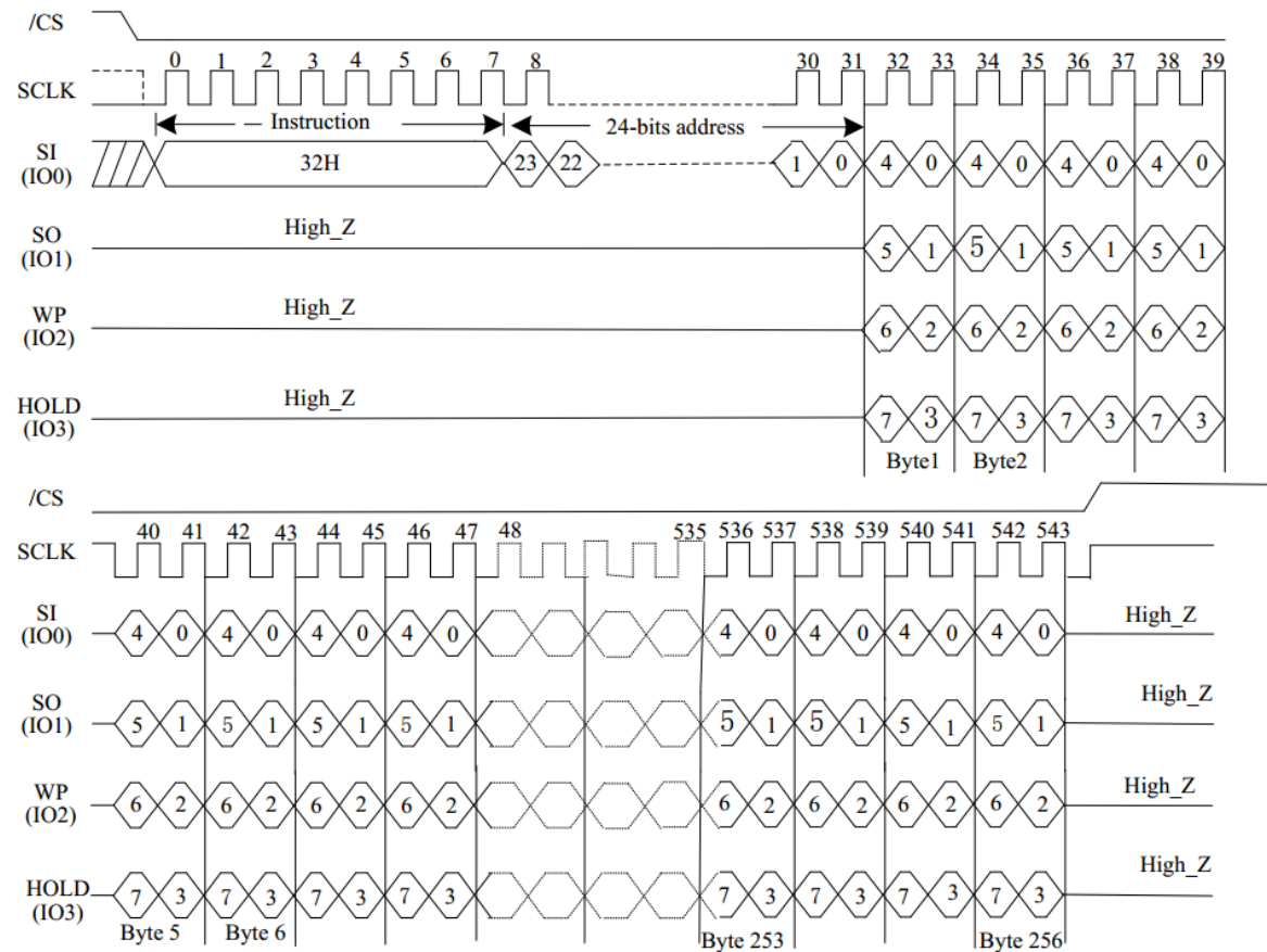
Figure 35. Qual Page Program Sequence Diagram
