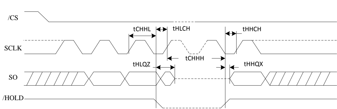
Figure 48. Hold Timing
