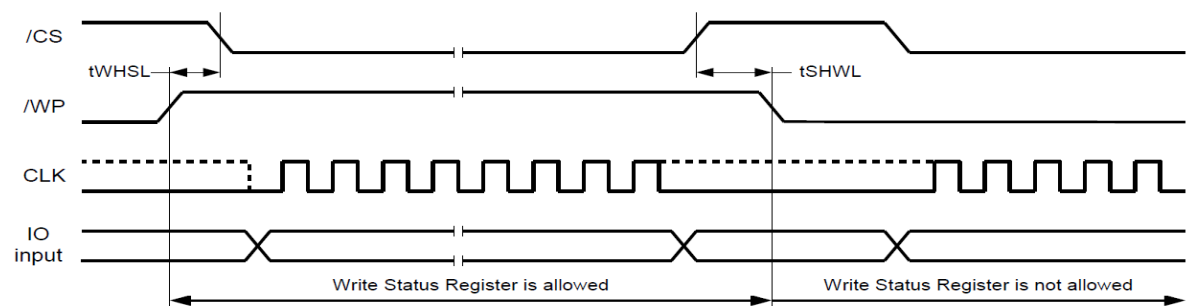
Figure 49. /WP Timing
